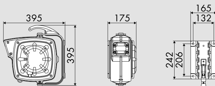
Overall dimensions with bayonet bracket (mm)
